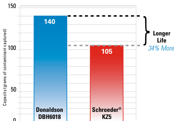
Contaminant Holding Capacity 3 5 \mu m
