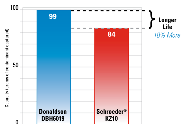
Contaminant Holding Capacity 4 10 \mu m
