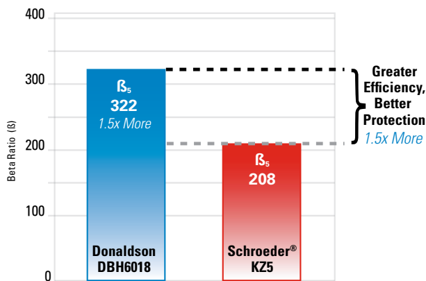
Beta Ratio ( \beta ) @ 5 \mu m particle size 1
