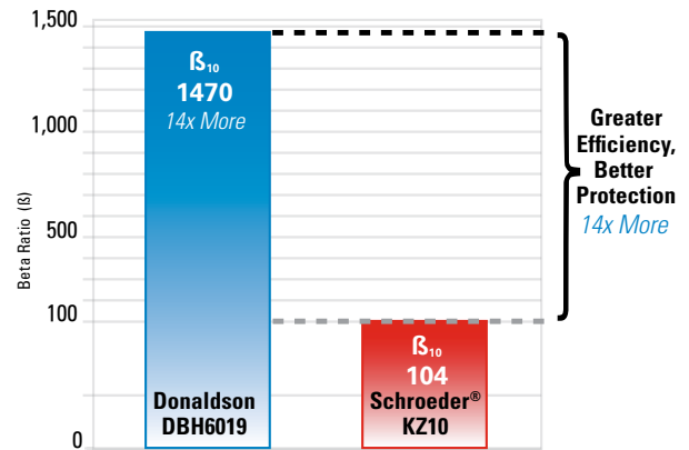
Beta Ratio ( \beta ) @ 10 \mu m particle size 2
