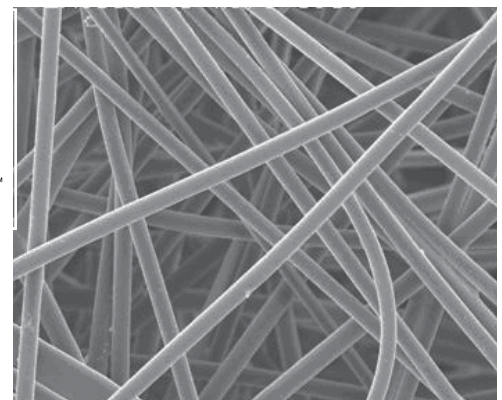
Scanning electron microscope image of Synteq XP™ at 300 magnification shows the uniform, resin-free fiber structure that allows increased filtration performance.
